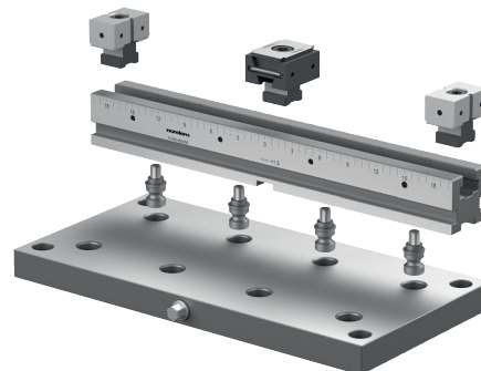
Adaptation of the multi-clamping system to a mechanical zero-point clamping system. Fits on 96mm gauge size. \text{Ø}16\text{H6} locating hole and M10 fastening thread.
